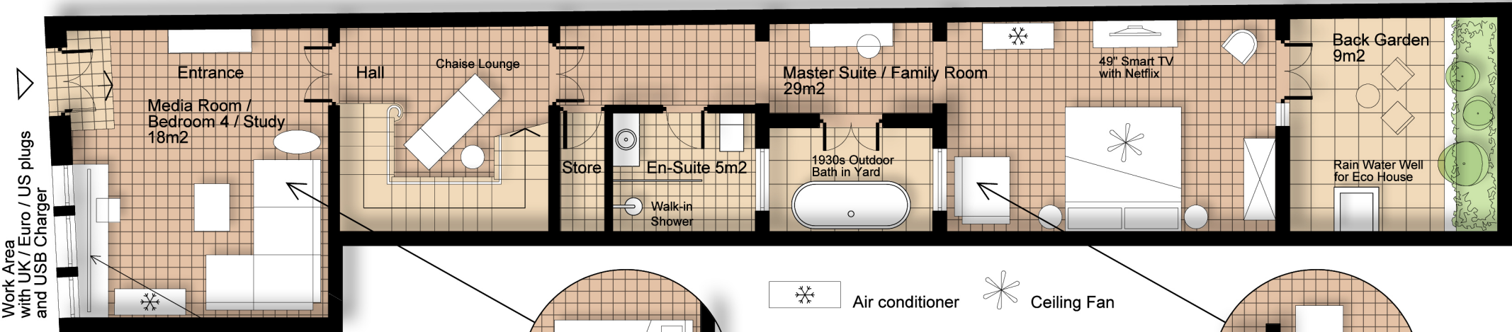
Ground Floor
